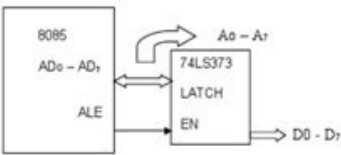
Fig. Demultiplexing of address and data lines in 8085 processor
